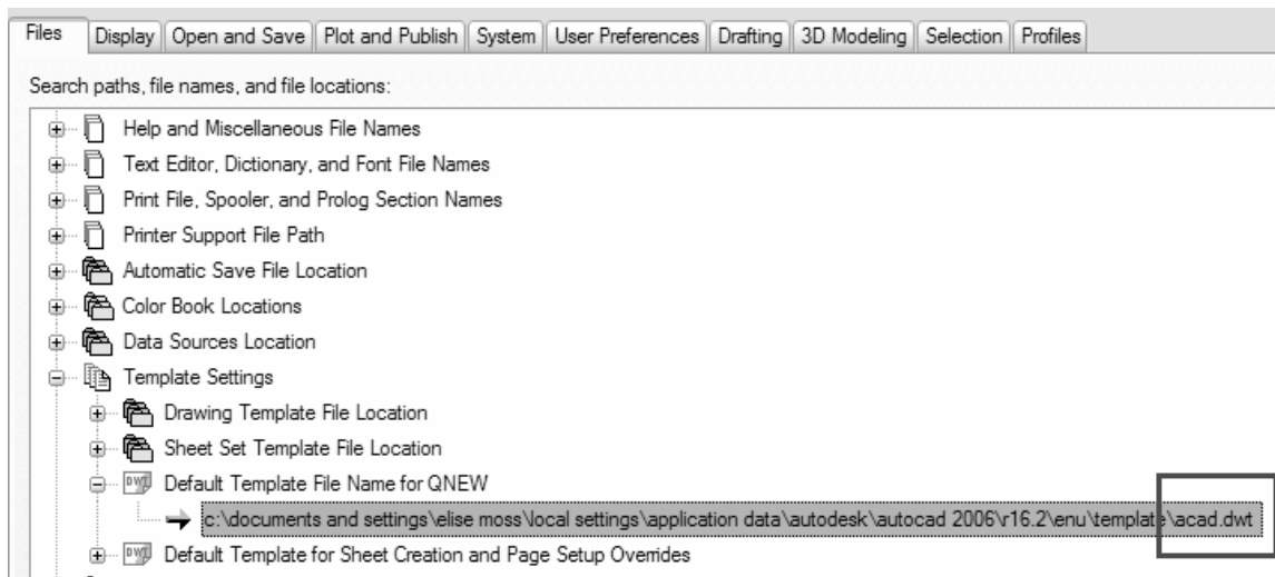
Figure 1 – The Options Dialog
